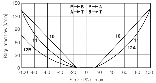
SDKZE 10 = L5 11 = S5 12A = D5 (P → A, A → T) 12B = D5 (P → B, B → T)
