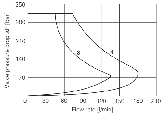
3 = spool S3, L3, D3 4 = spool S5, L5, D5
