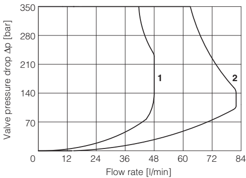
1 = spool L3, S3, D3 2 = spool L5, S5, D5
